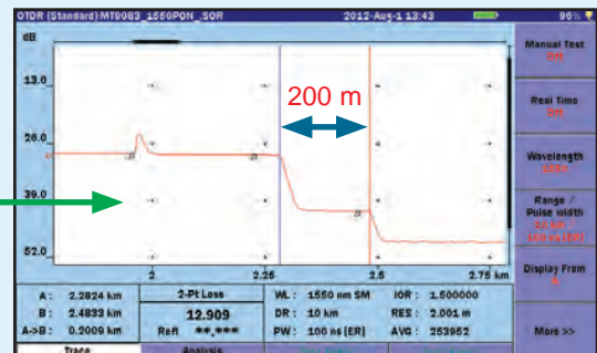
Fig 1: Typical PON 1 × 64 count System Measurement from the customer premise.
