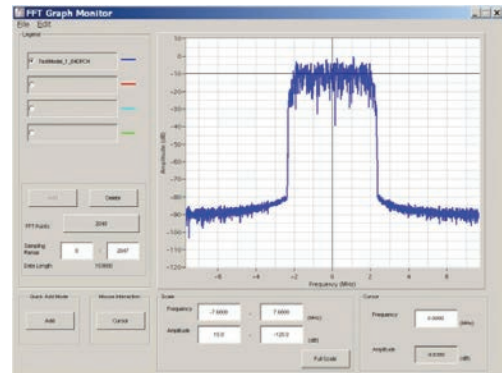
FFT Screen
