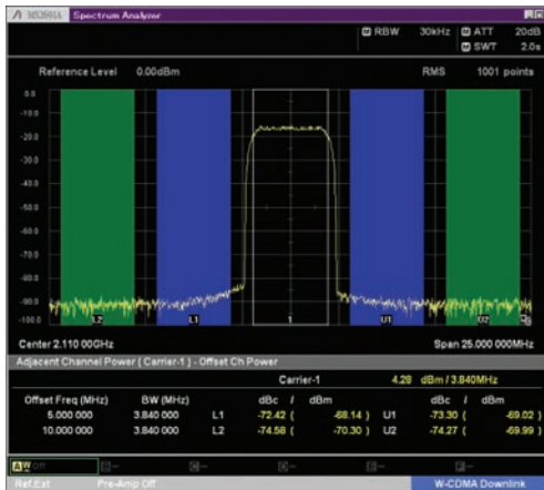
W-CDMA ACLR (1 Carrier) Waveform Pattern (TestModel1, 64DPCH)
