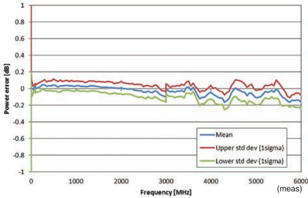
Frequency Characteristic
